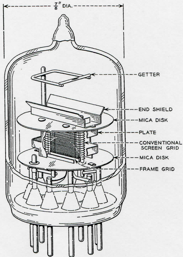
Fig. 9—Cutaway view of the 435A.
