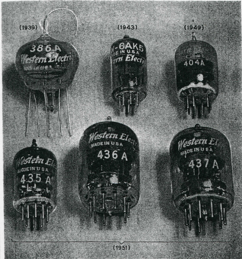
Fig. 8—The 386A, 408A, 404A, 435A, 436A and the 437A tubes approximately actual size.
