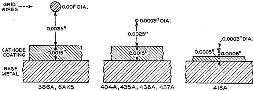
Fig. 5—Trend in spacing and grid wire size.
